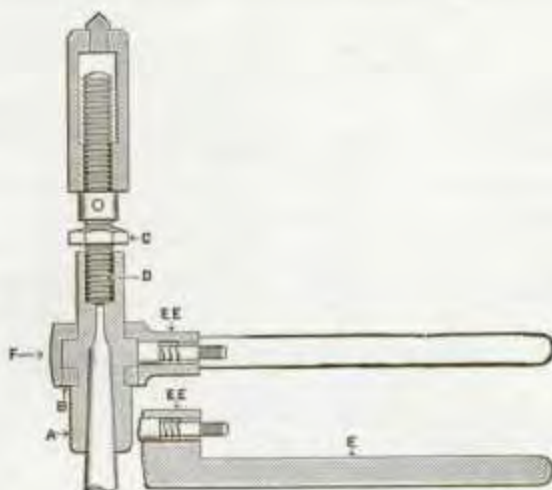
Sectional View of Whitney Reversible Ratchet Drills.
