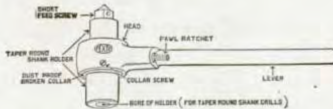
Ratchet Drill Complete with Short Feed Screw and Holder for Taper Round Shank Drills
