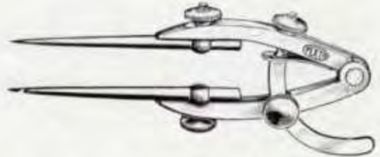
DOUBLE LEG, TWO MOVABLE POINTS
